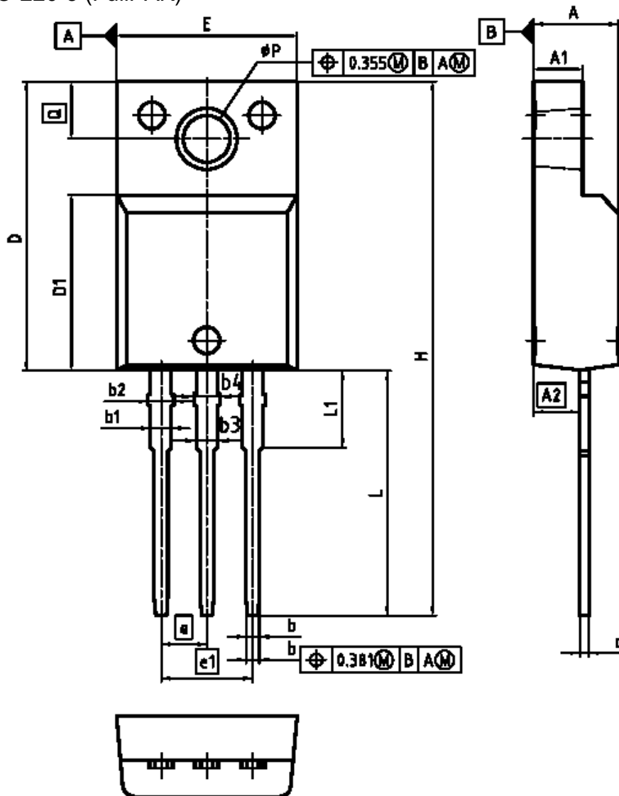
PG-TO-220-3 (FullPAK)
